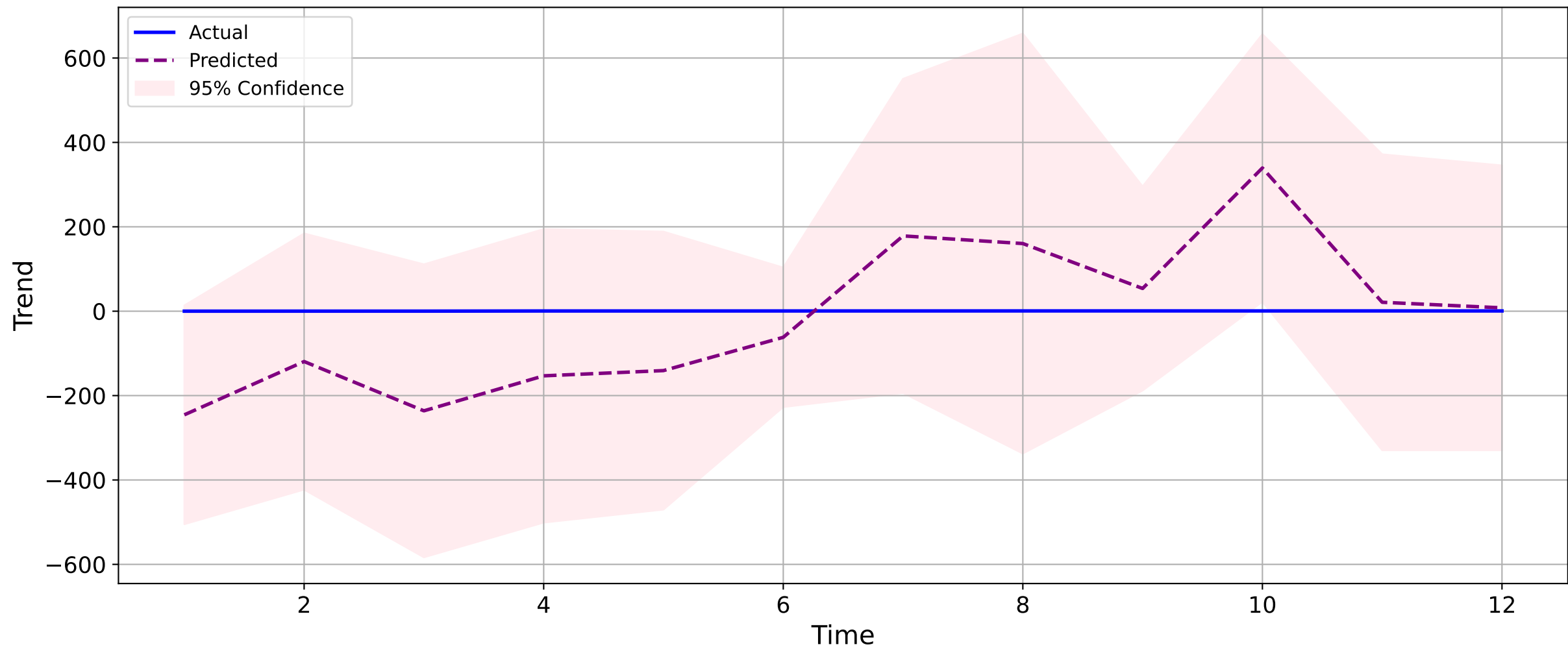
Defacement-ALL - Validation
